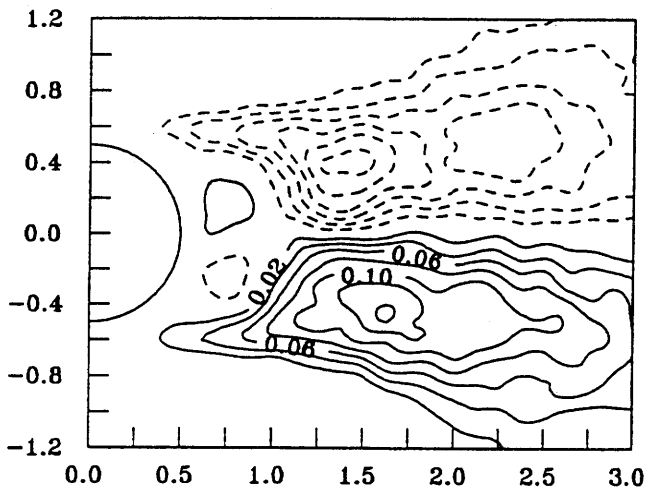
Base cylinder
